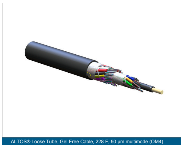
ALTOS® Loose Tube, Gel-Free Cable, 228 F, 50 µm multimode (OM4)
