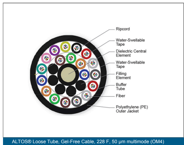
ALTOS® Loose Tube, Gel-Free Cable, 228 F, 50 µm multimode (OM4)
